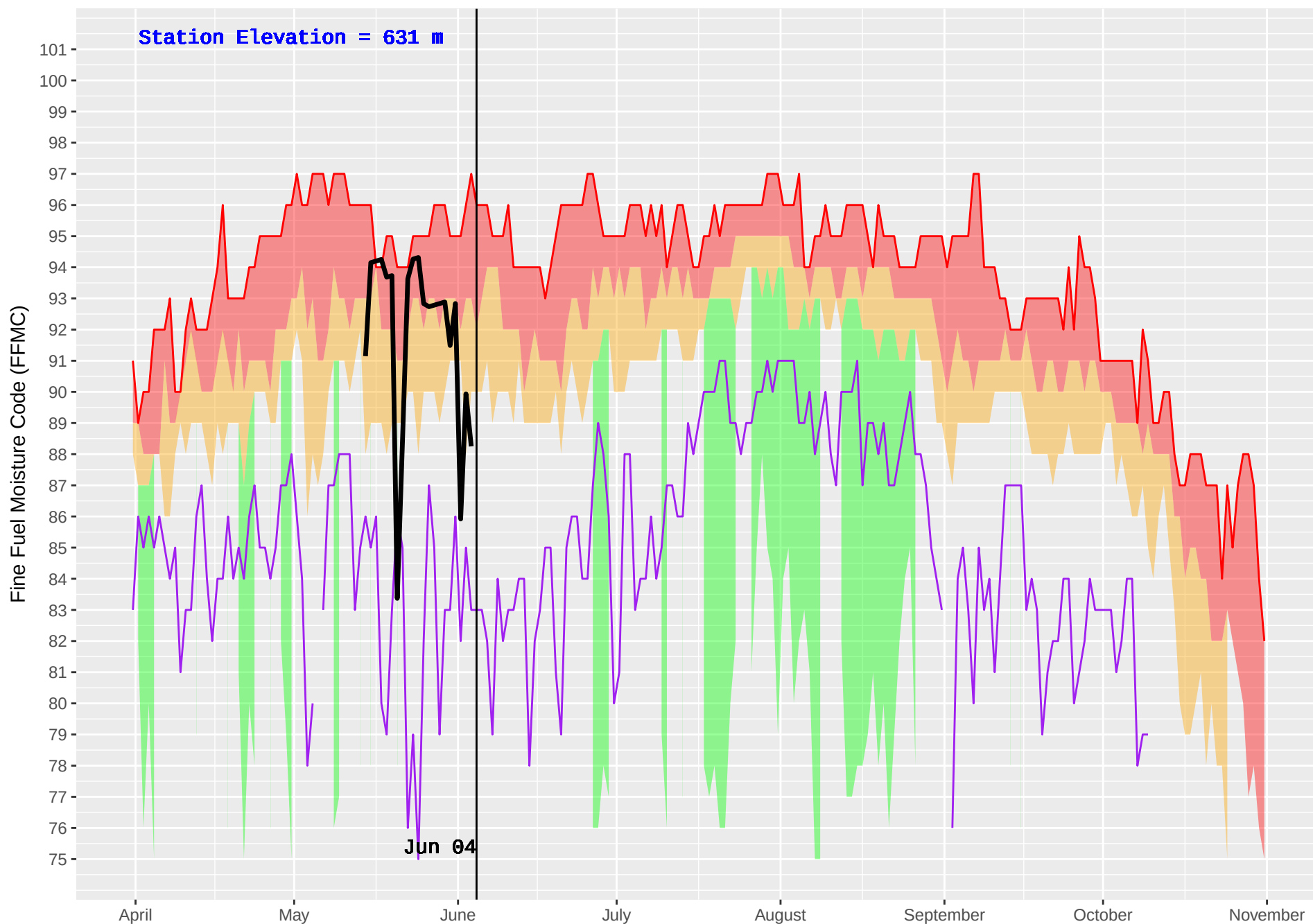
EAST BARRIERE (243) : Historical (1978–2016) and Current (2018) Noon Fine Fuel Moisture Code (FFMC)
