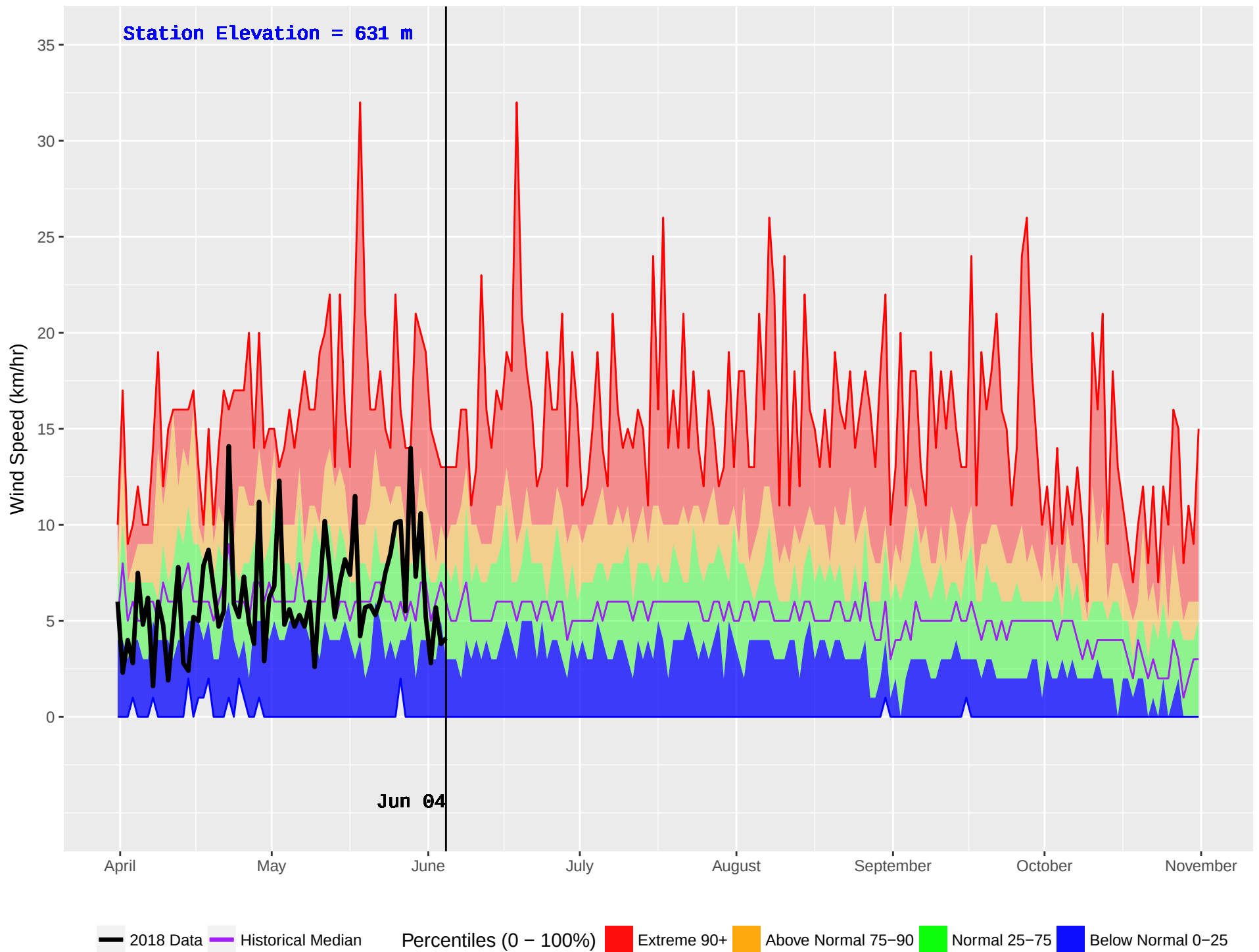
EAST BARRIERE (243) : Historical (1978–2016) and Current (2018) Noon Wind Speed
