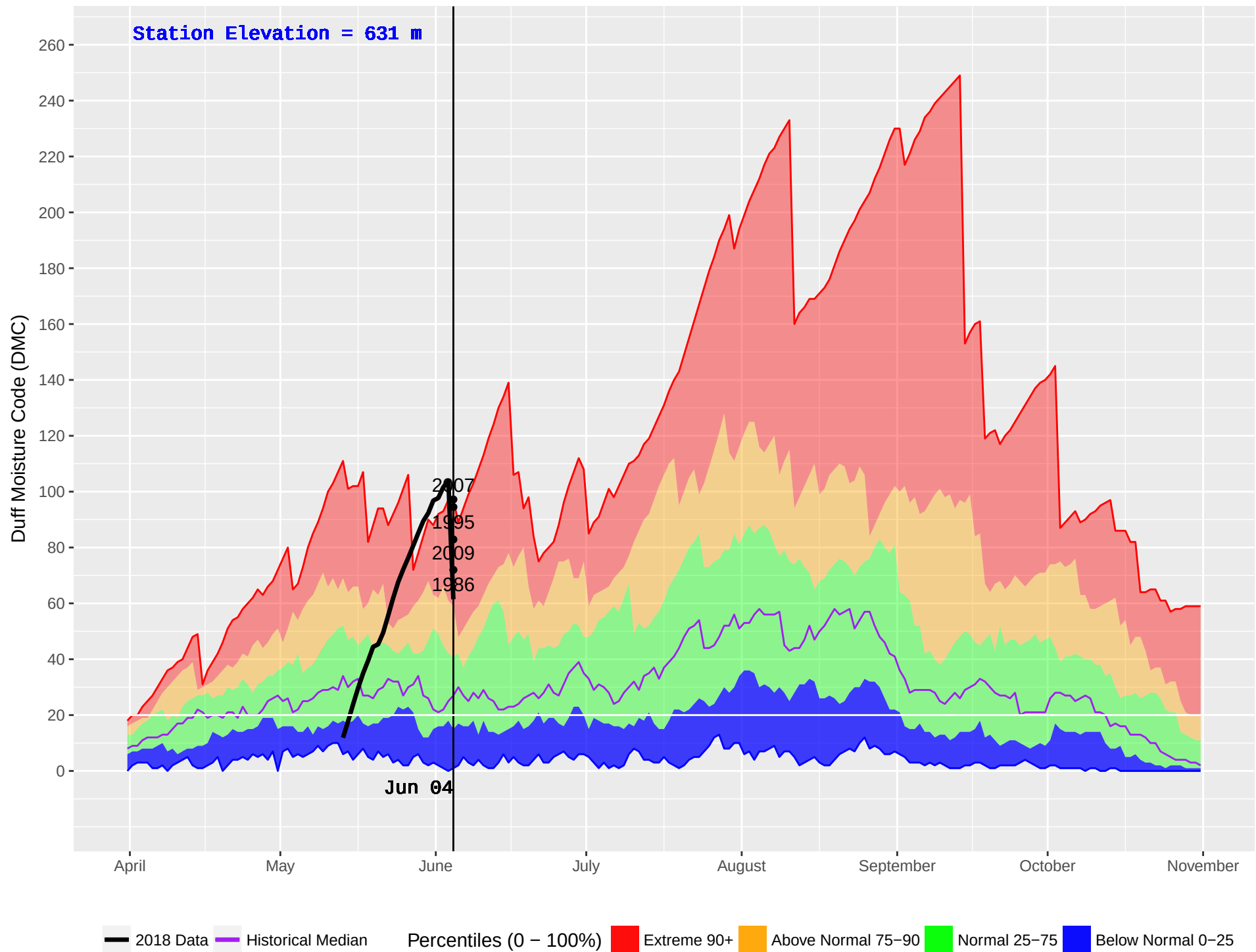
EAST BARRIERE (243) : Historical (1978–2016) and Current (2018) Noon Duff Moisture Code (DMC)
