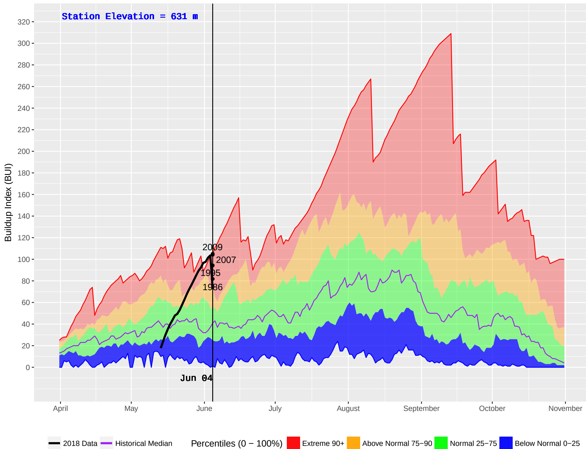
EAST BARRIERE (243) : Historical (1978–2016) and Current (2018) Noon Buildup Index (BUI)
